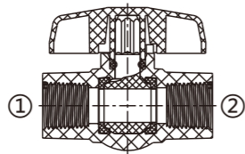
COMPACT BALL VALVE W/EPDM O-RING (FIPT x FIPT)
