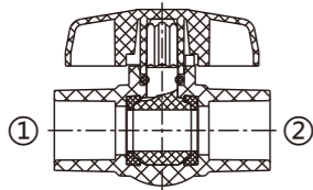
COMPACT BALL VALVE W/EPDM O-RING (SOC x SOC)
